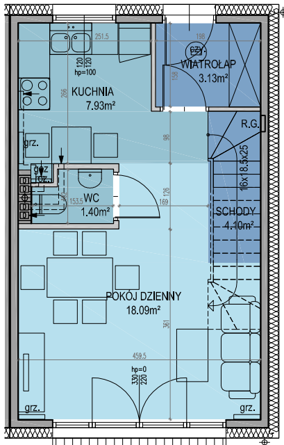
PARTER
